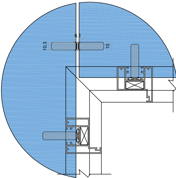
DETAY-3.4
