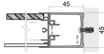
5-DETAY
