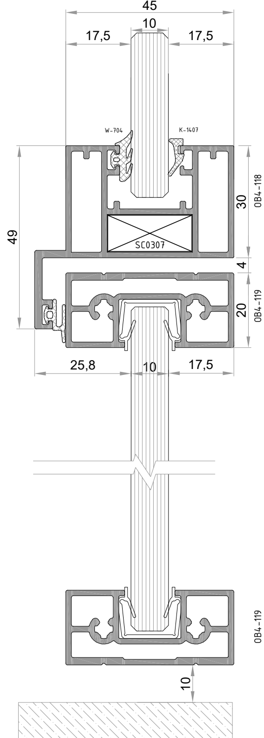
DETAY-5
