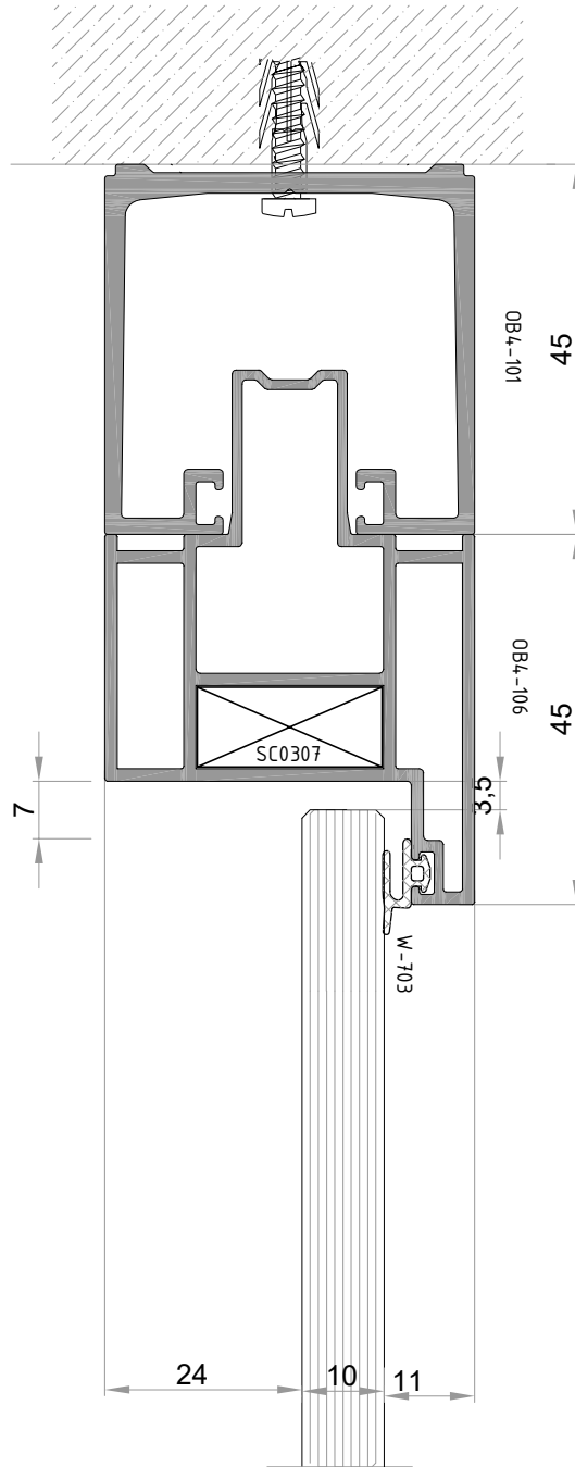
DETAY-1
