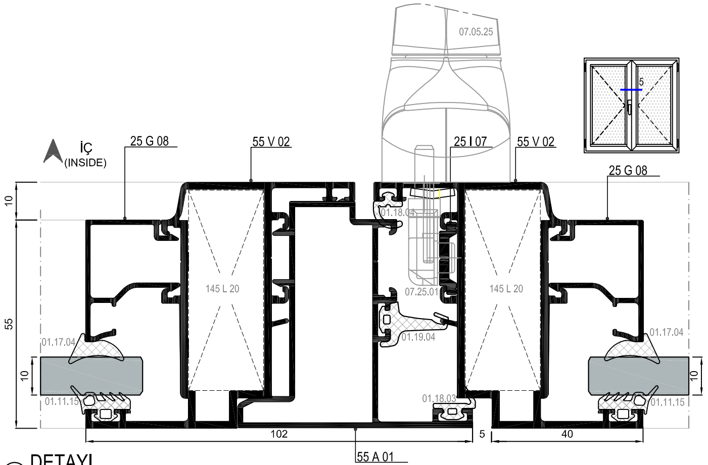
⑤ DETAYI DETAIL
