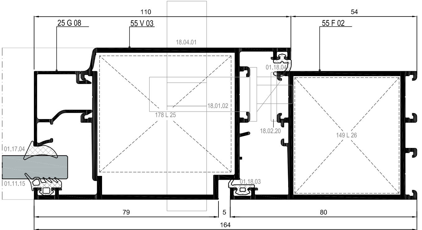
20 DETAYI DETAIL
