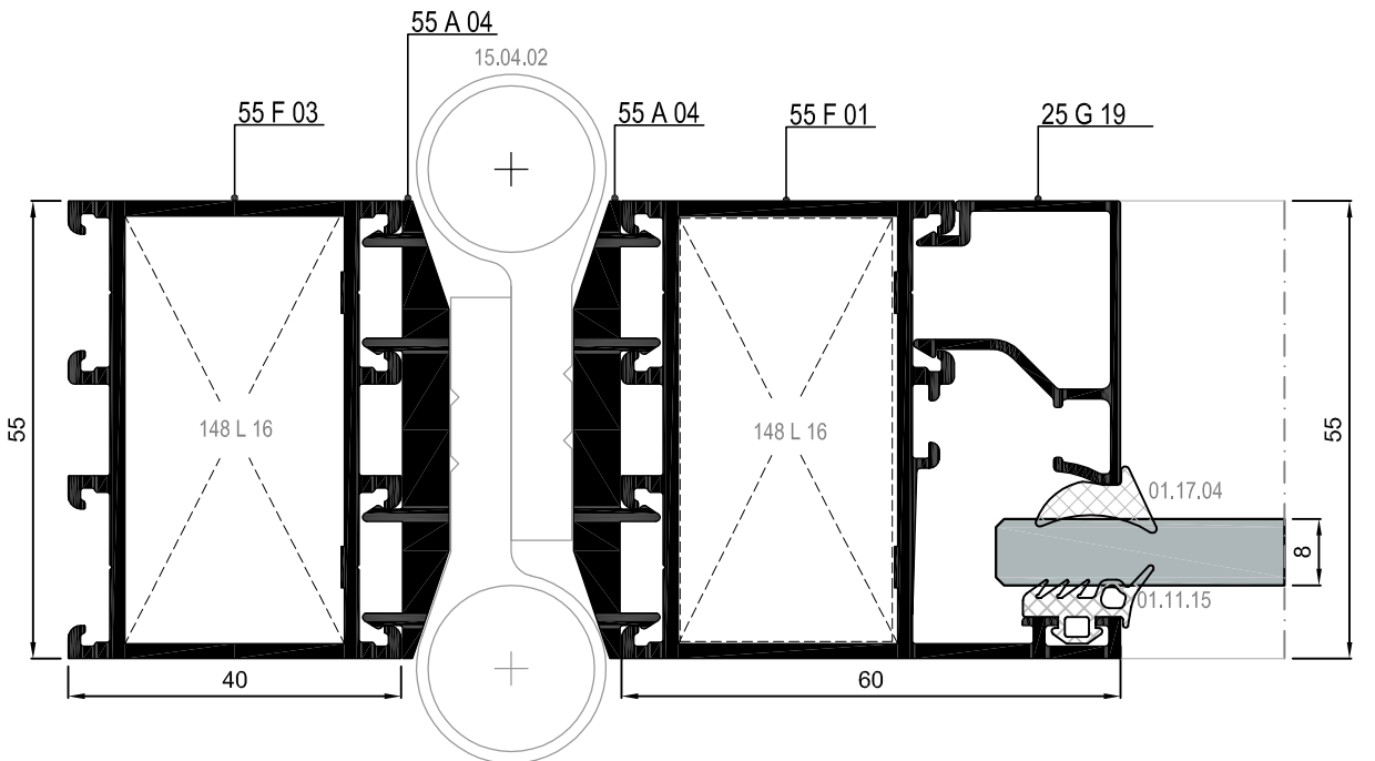
⑭ DETAYI DETAIL
