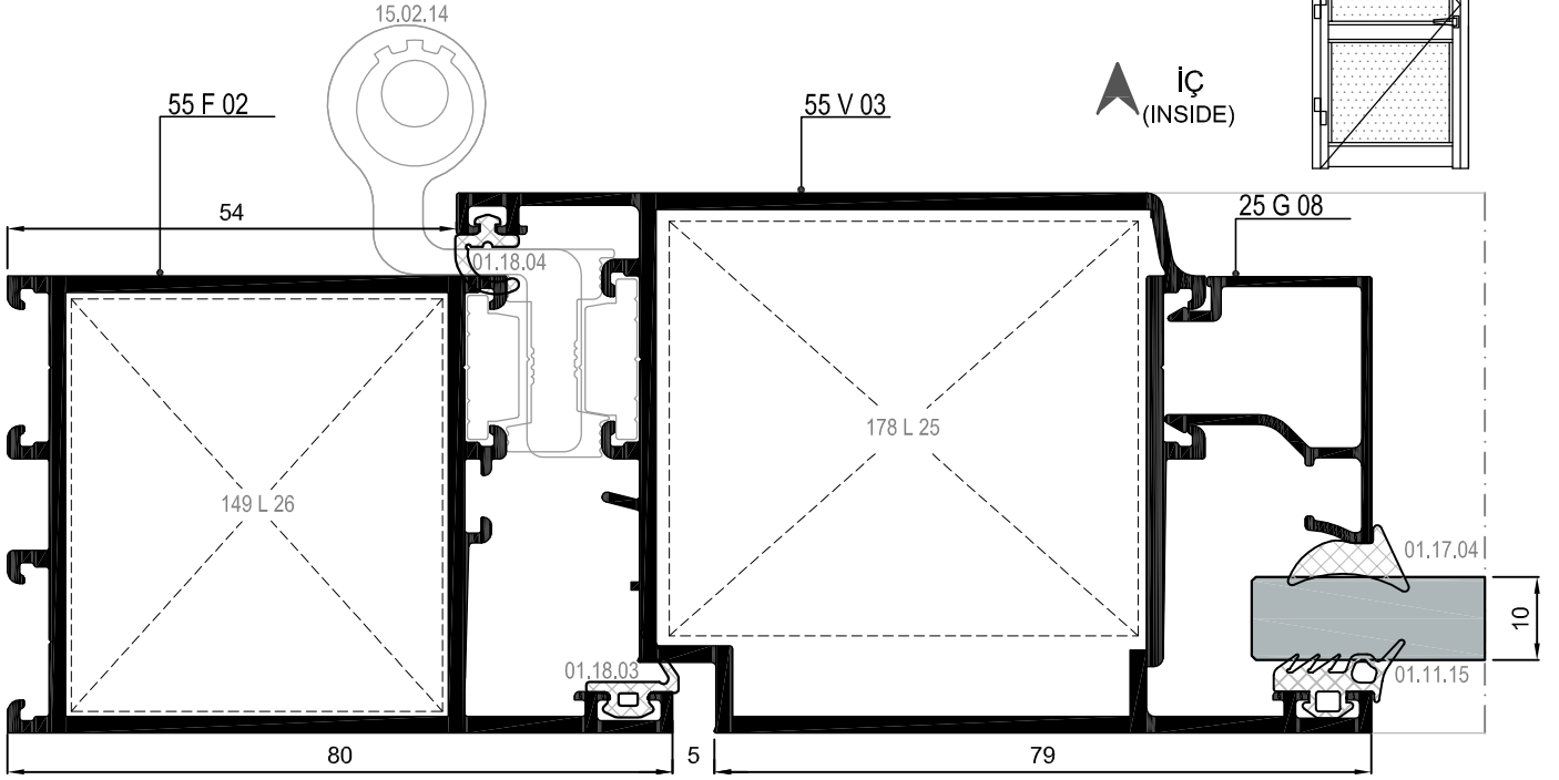
19 DETAYI DETAIL
