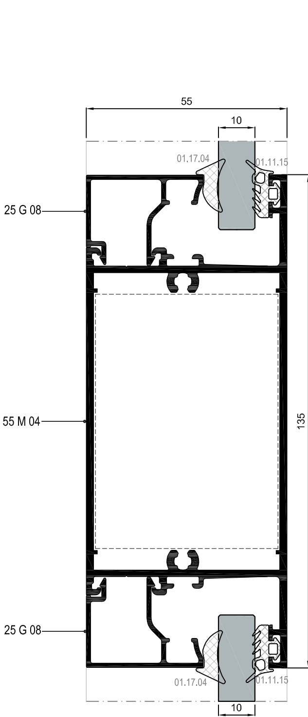
22 DETAYI DETAIL
